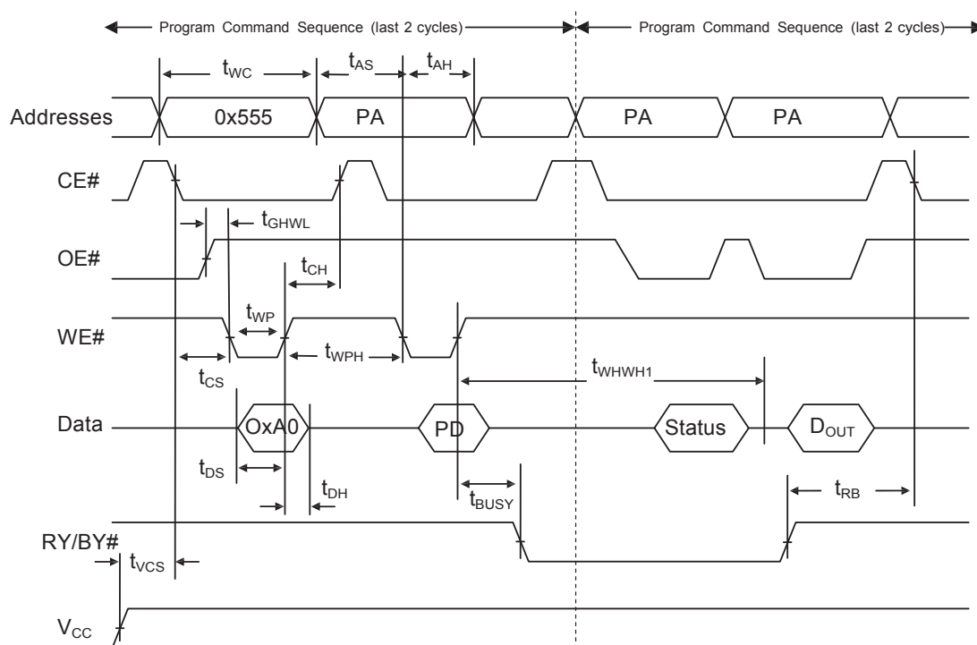
Figure 5. Program Operation Timings
