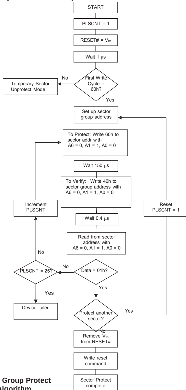
Flowchart 7a. In-System Sector Group Protect Flowchart
