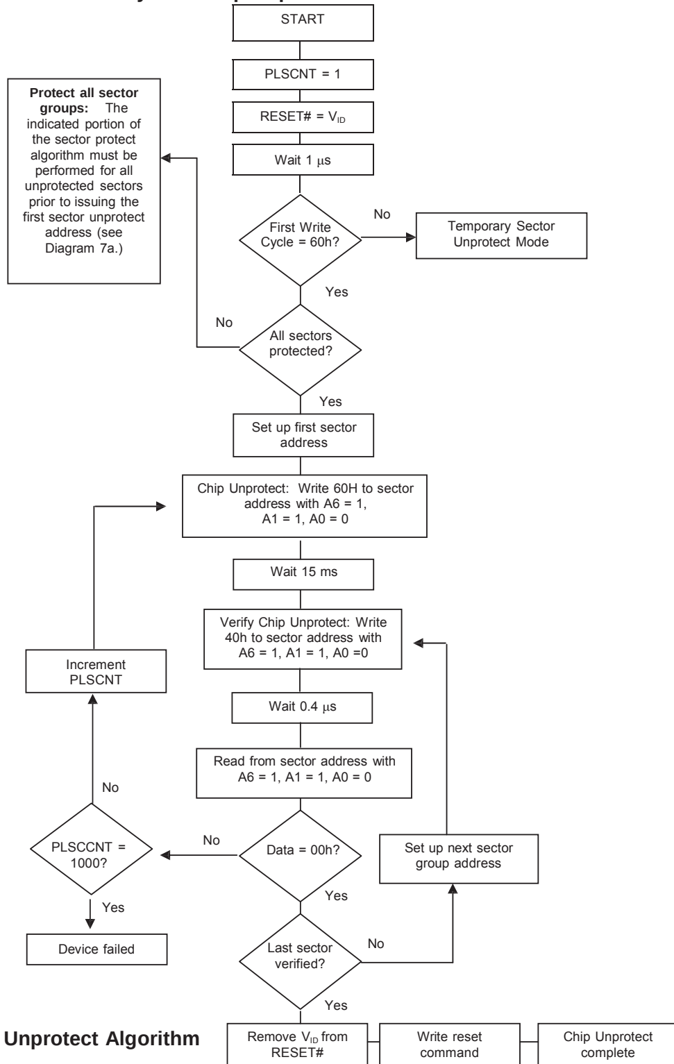
Flowchart 7b. In-System Chip Unprotect Flowchart
