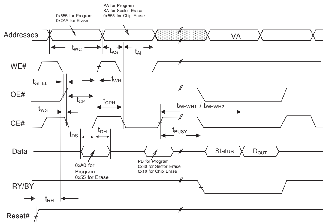
Figure 8. Alternate CE# Controlled Write Operation Timings
